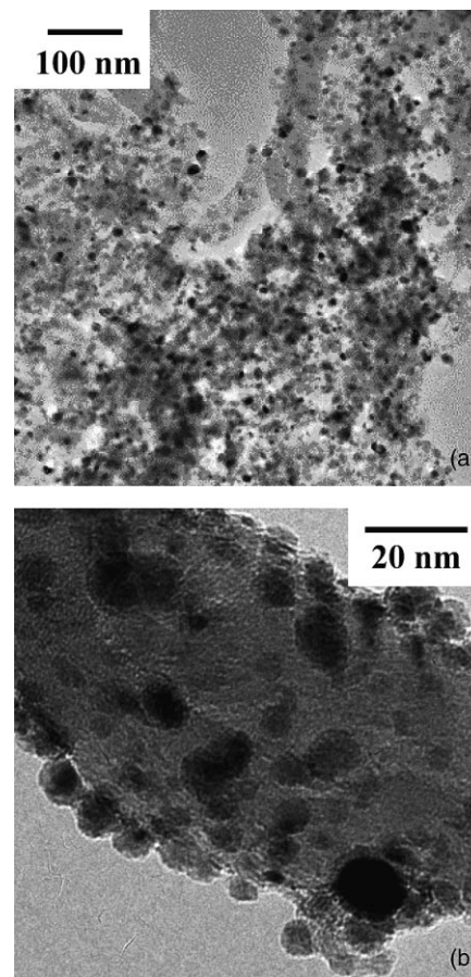
Figure 1. TEM micrograph of reduced 10 wt% Ni/CNF prepared via HDP: (a) low magnification and (b) high magnification.
