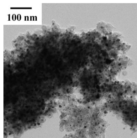
Figure 4. TEM of reduced 45 wt% Ni/CNF-ox prepared via incipient wetness.
