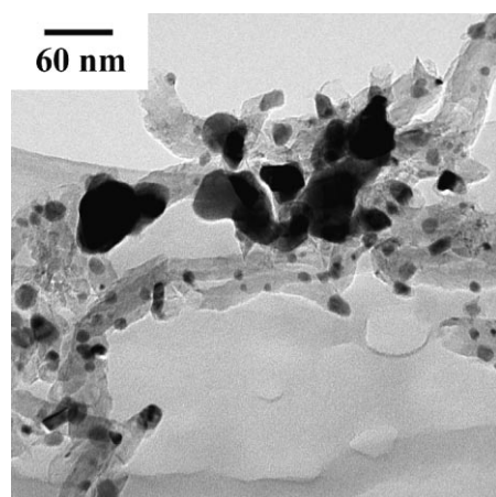
Figure 3. TEM of reduced 30 wt% Ni/CNF-ox prepared via incipient wetness impregnation.
