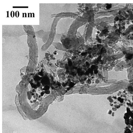
Figure 2. TEM of reduced 10 wt% Ni/CNF-as prepared by HDP.
