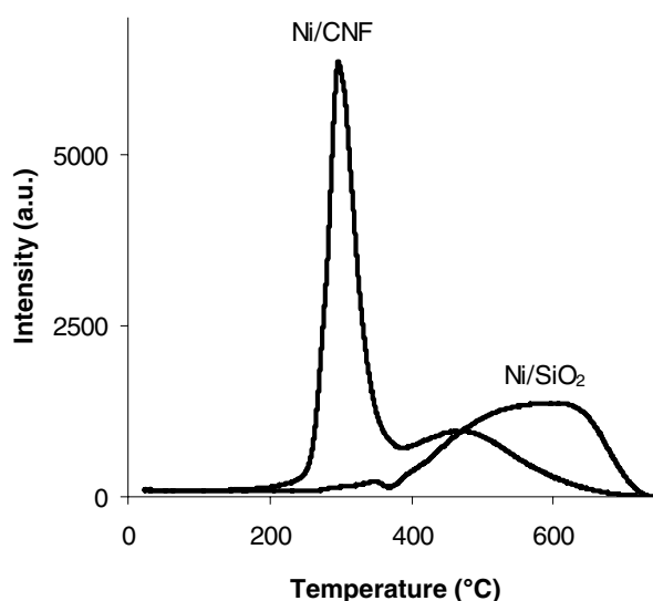
Figure 5. TPR results of 50 wt% Ni/SiO 2 and 45 wt% Ni/CNF.
